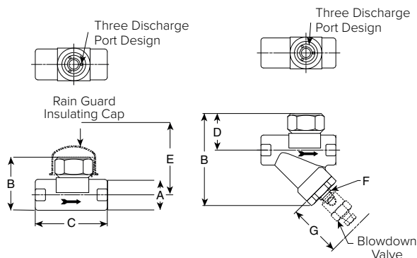
CD-33/CD-33L Series
